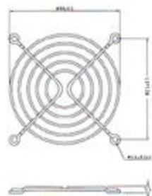
6G-92 for 92mm fan
